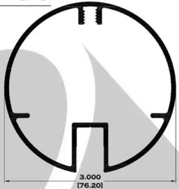
2830 PASAMANOS REDONDO 3"
