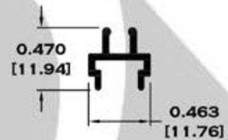
10554 MOSQUITERO
