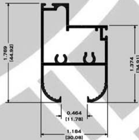
2231 MARCO COLONIAL
