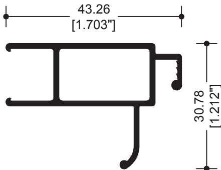
7112 VERTICAL MOSQUITERO
